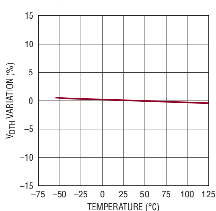
Discharge Threshold Variation vs Temperature
