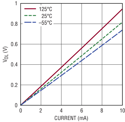
V_{OL} vs Output Sink Current RSTB, FAULTB, ALERTB
