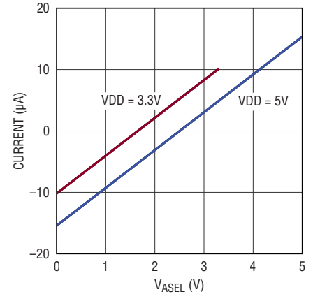
ASEL \overline{n} Current vs Input Voltage
