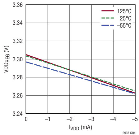
VDD Load Regulation
